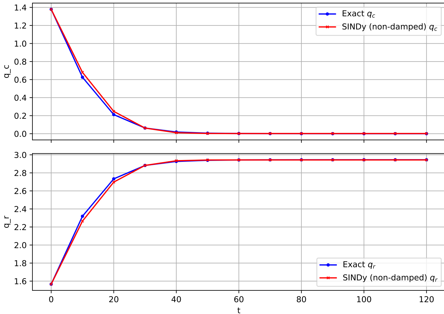
Trajectory 635 (non-damped)
