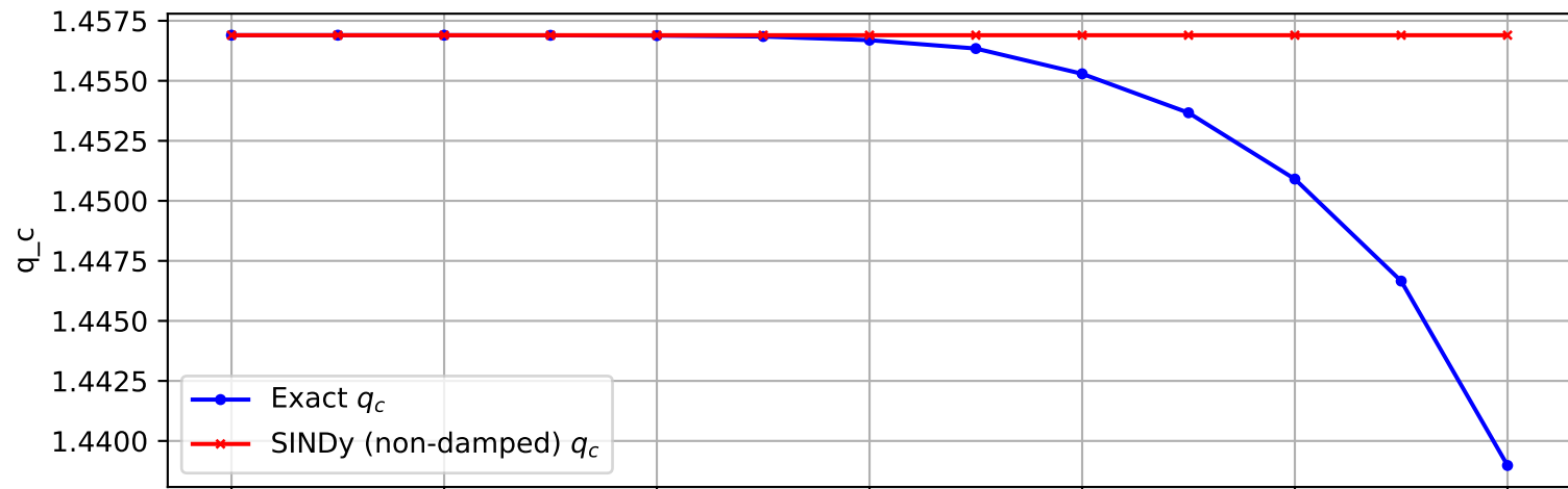
Trajectory 64 (non-damped)
