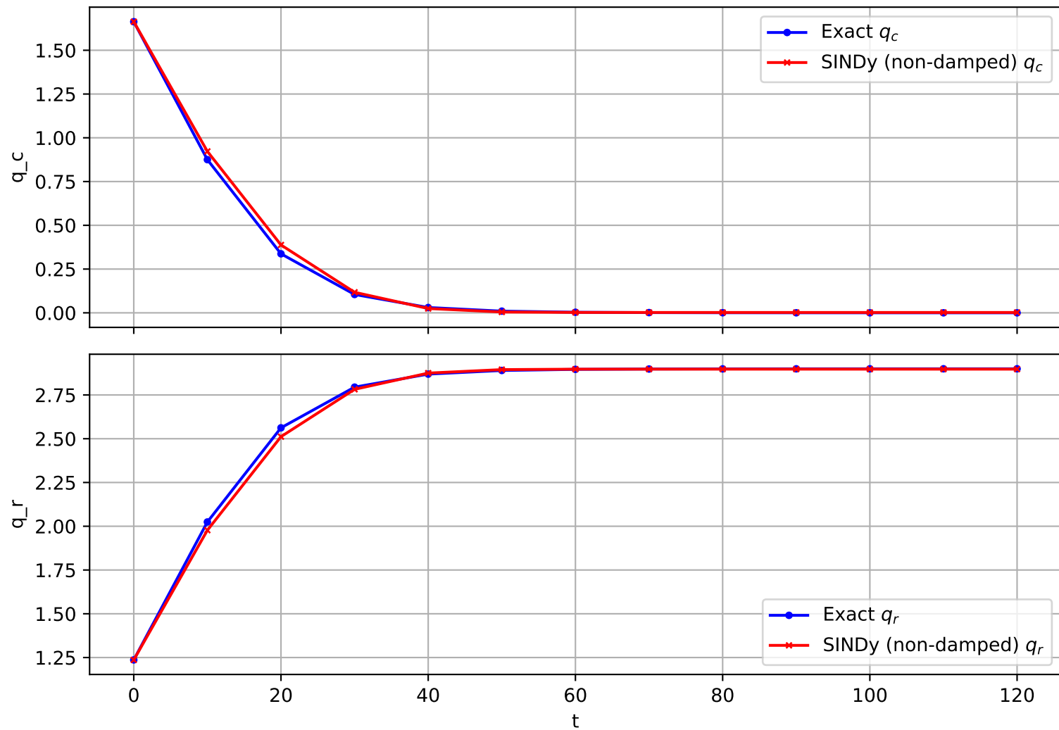
Trajectory 641 (non-damped)
