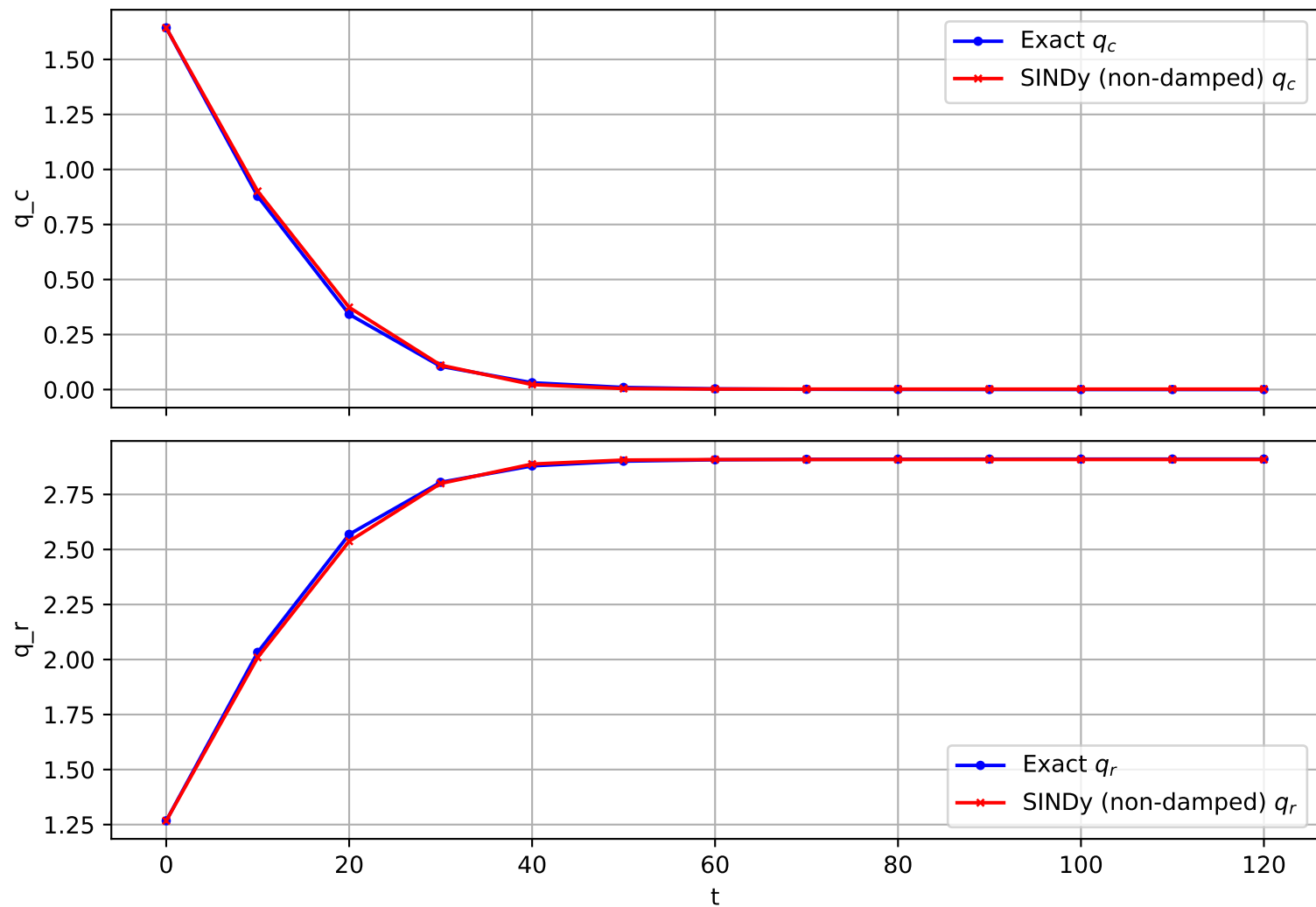
Trajectory 642 (non-damped)
