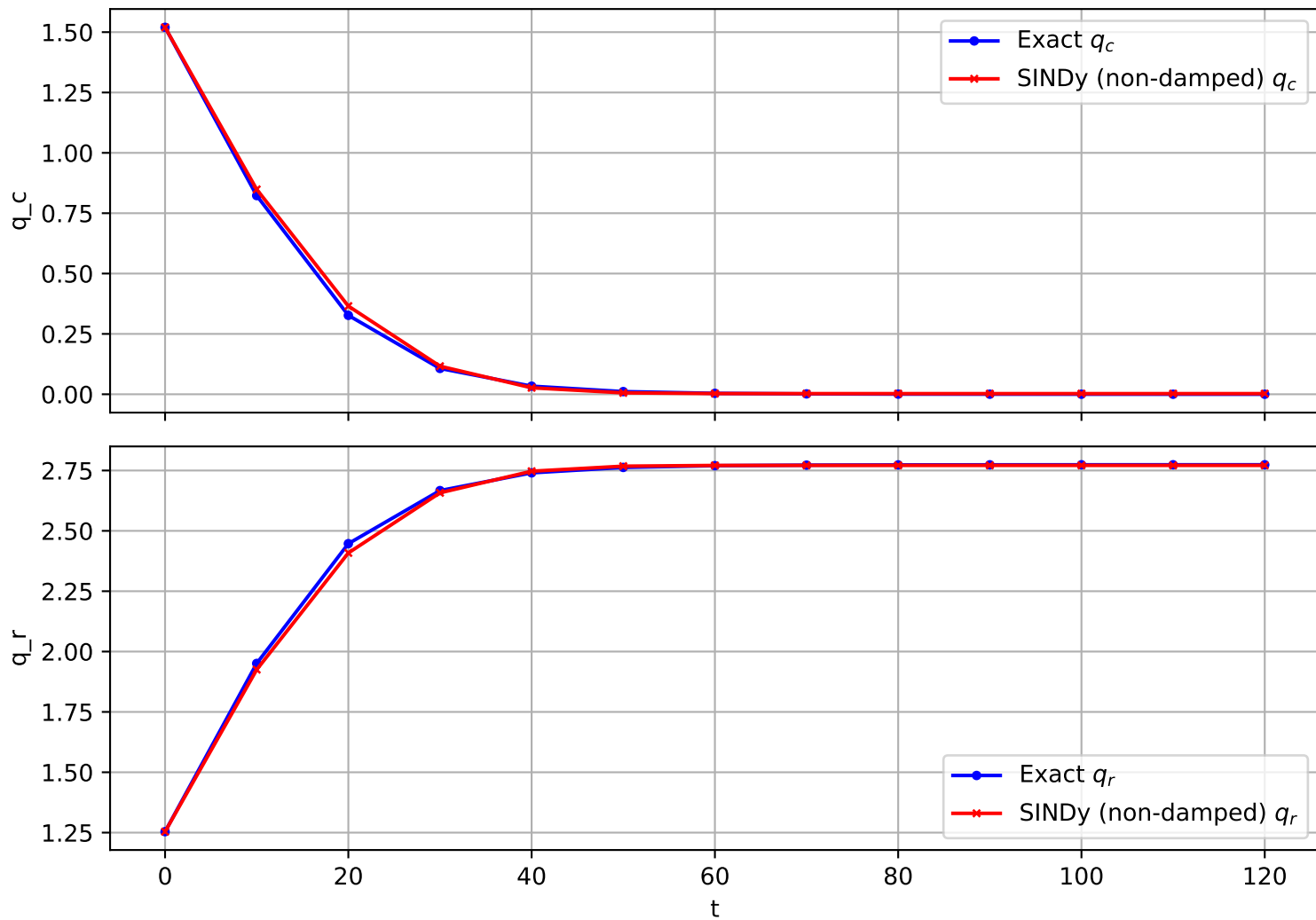
Trajectory 644 (non-damped)
