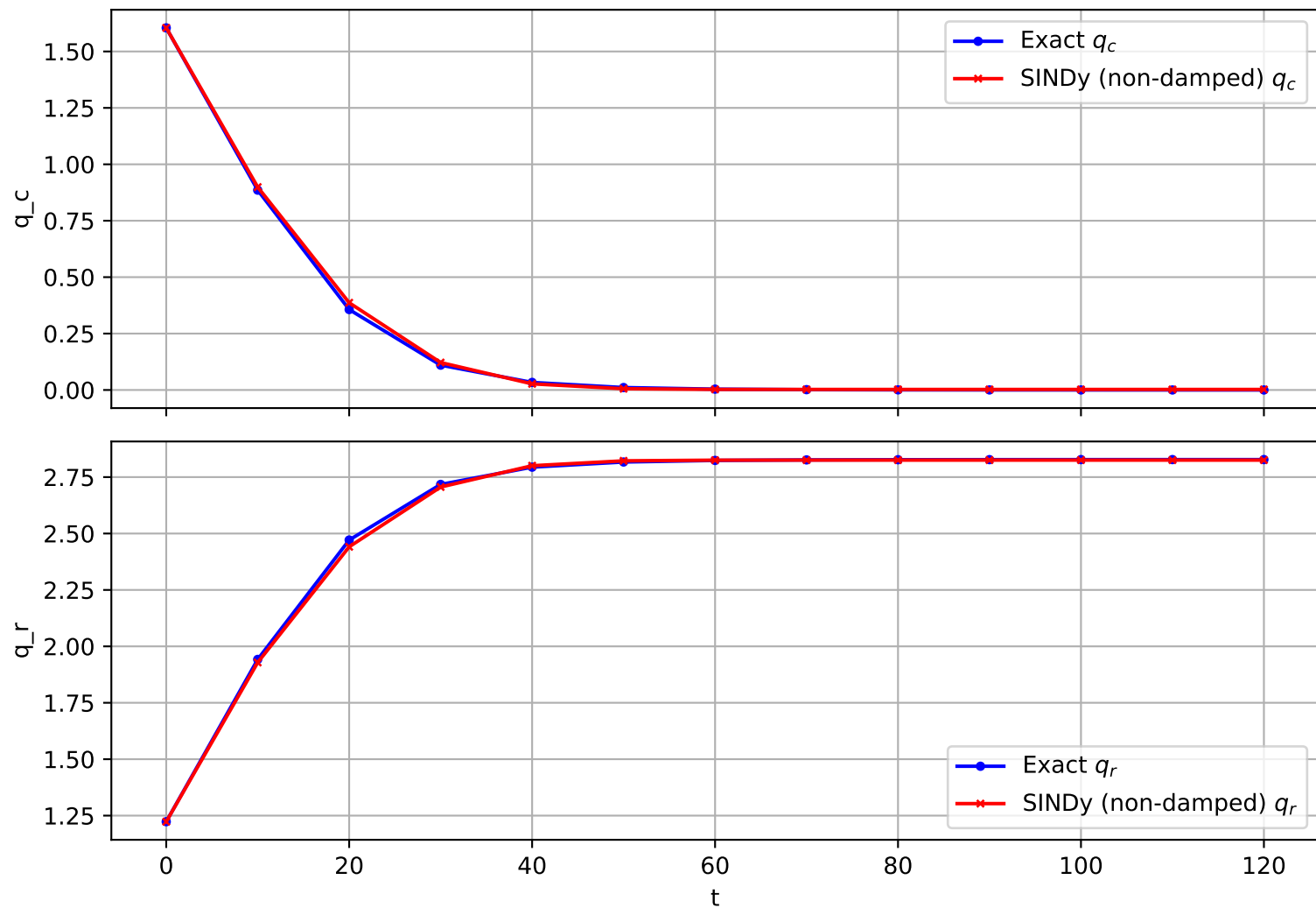
Trajectory 645 (non-damped)
