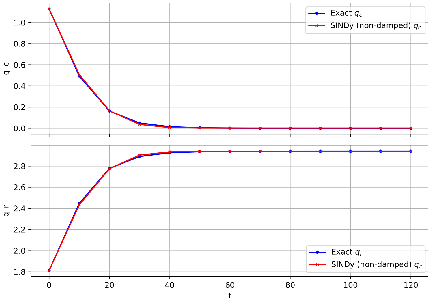
Trajectory 654 (non-damped)
