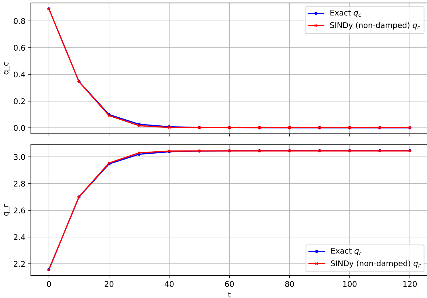
Trajectory 657 (non-damped)
