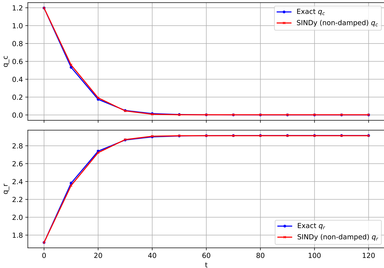
Trajectory 669 (non-damped)
