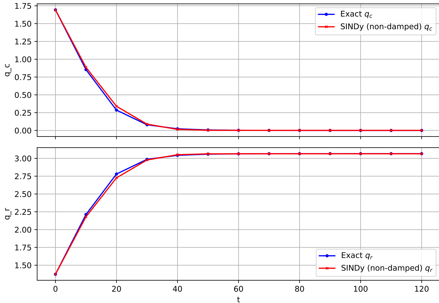
Trajectory 675 (non-damped)
