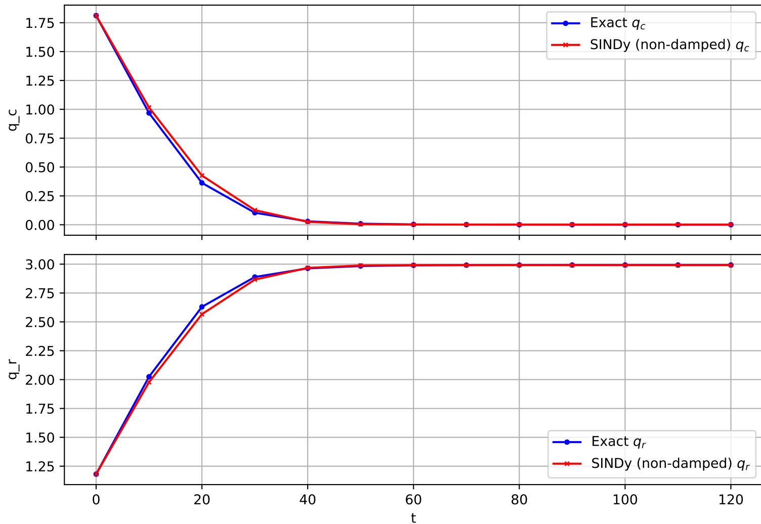
Trajectory 682 (non-damped)
