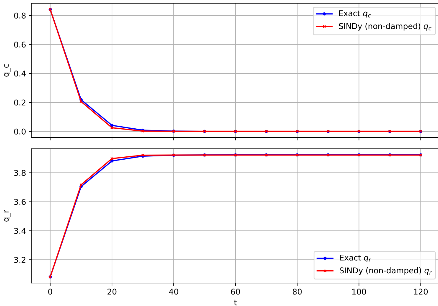
Trajectory 688 (non-damped)
