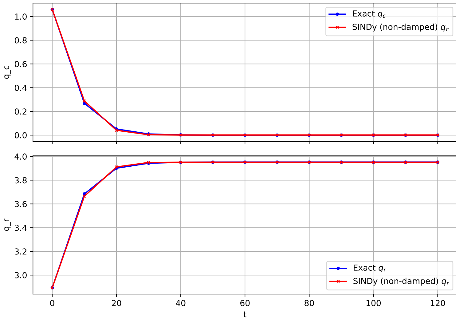
Trajectory 703 (non-damped)
