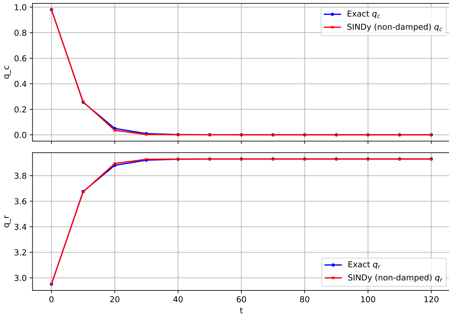
Trajectory 704 (non-damped)
