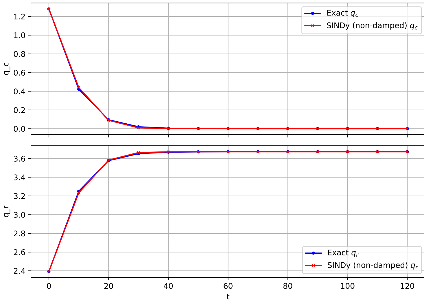
Trajectory 712 (non-damped)
