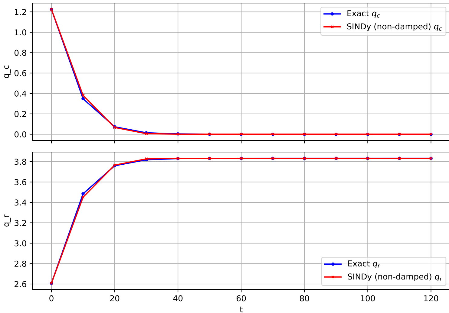
Trajectory 715 (non-damped)
