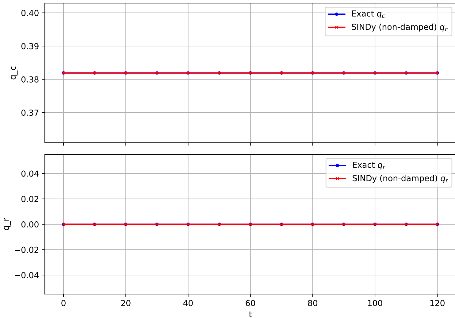
Trajectory 726 (non-damped)
