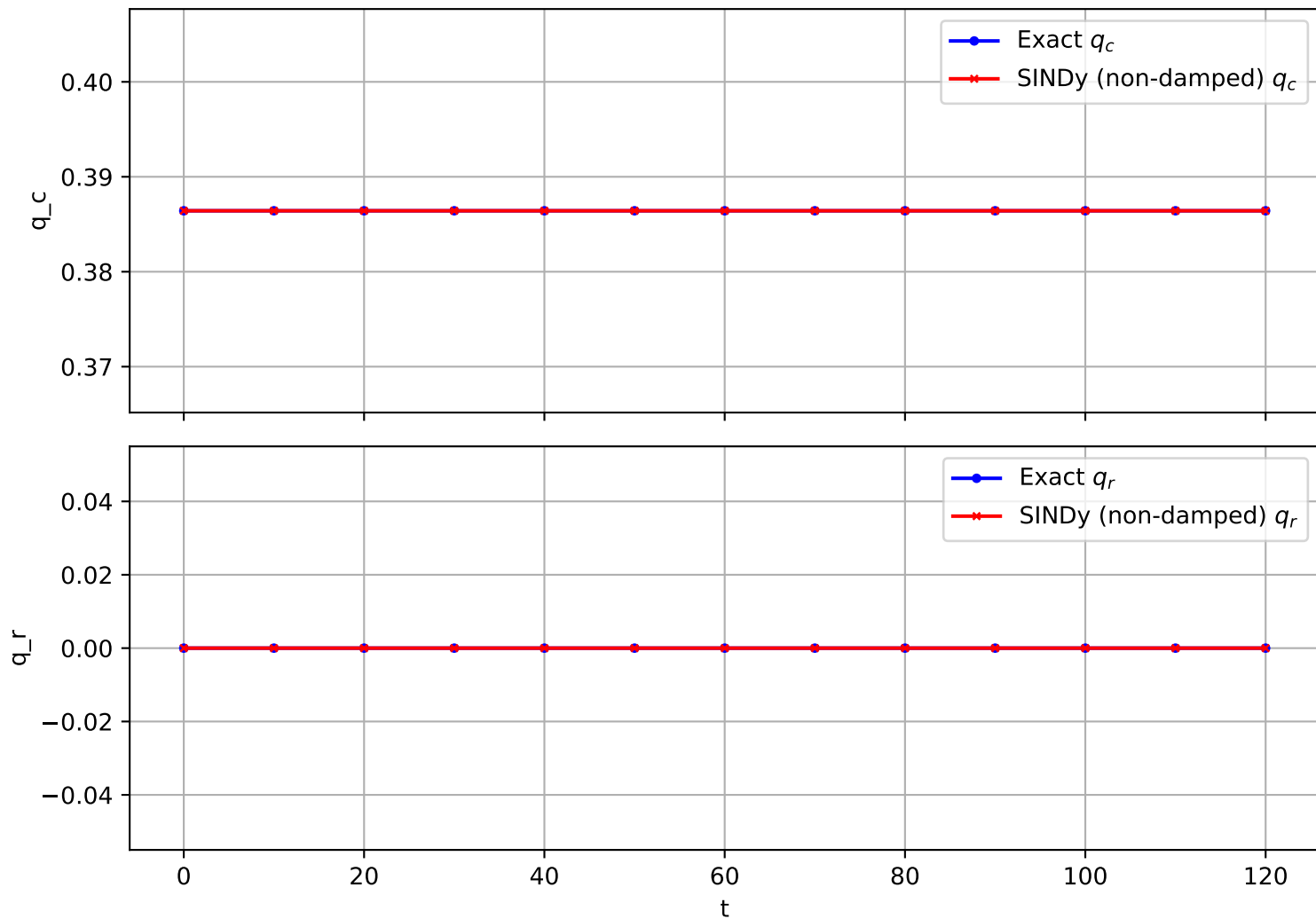
Trajectory 727 (non-damped)
