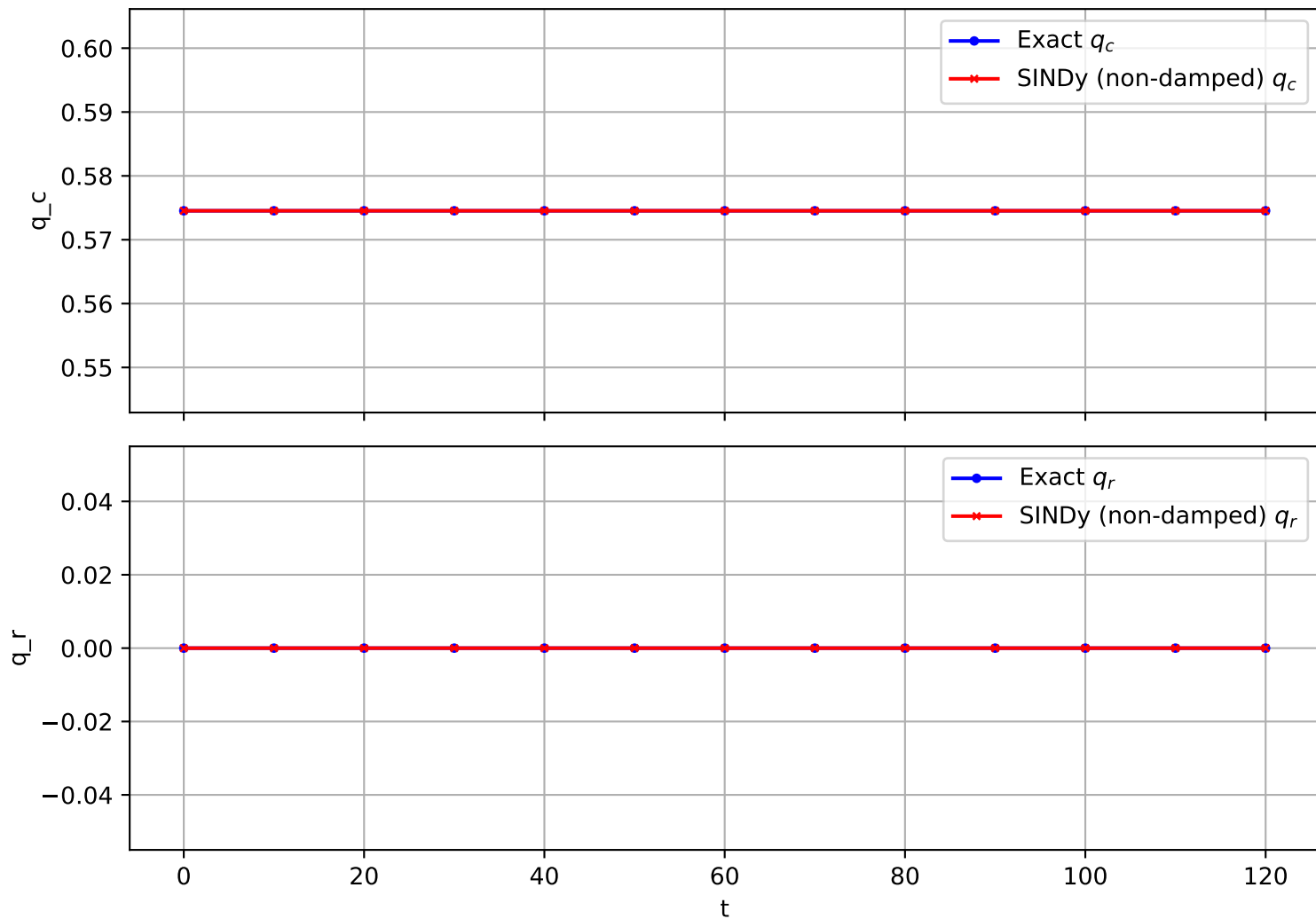
Trajectory 733 (non-damped)
