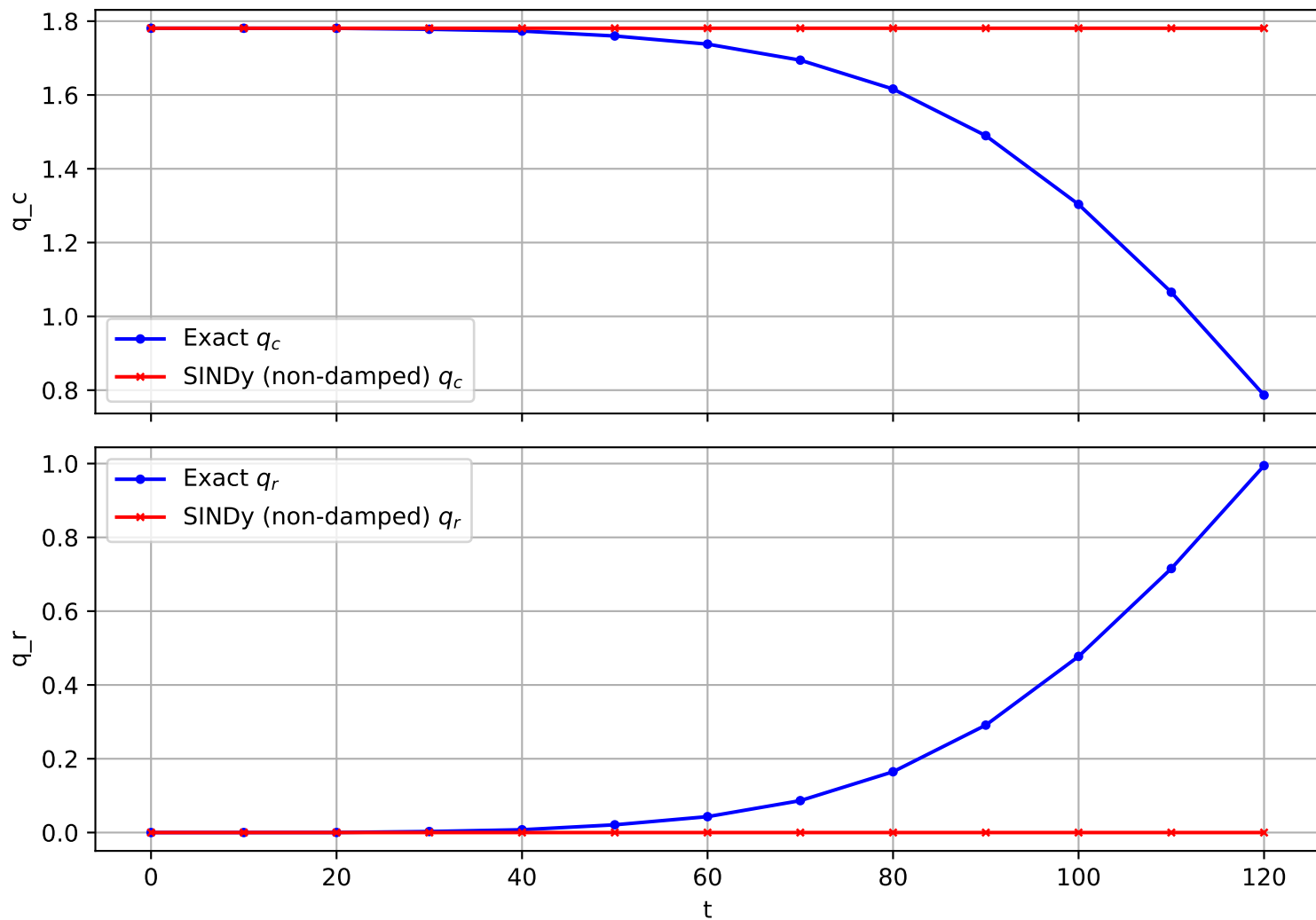
Trajectory 76 (non-damped)
