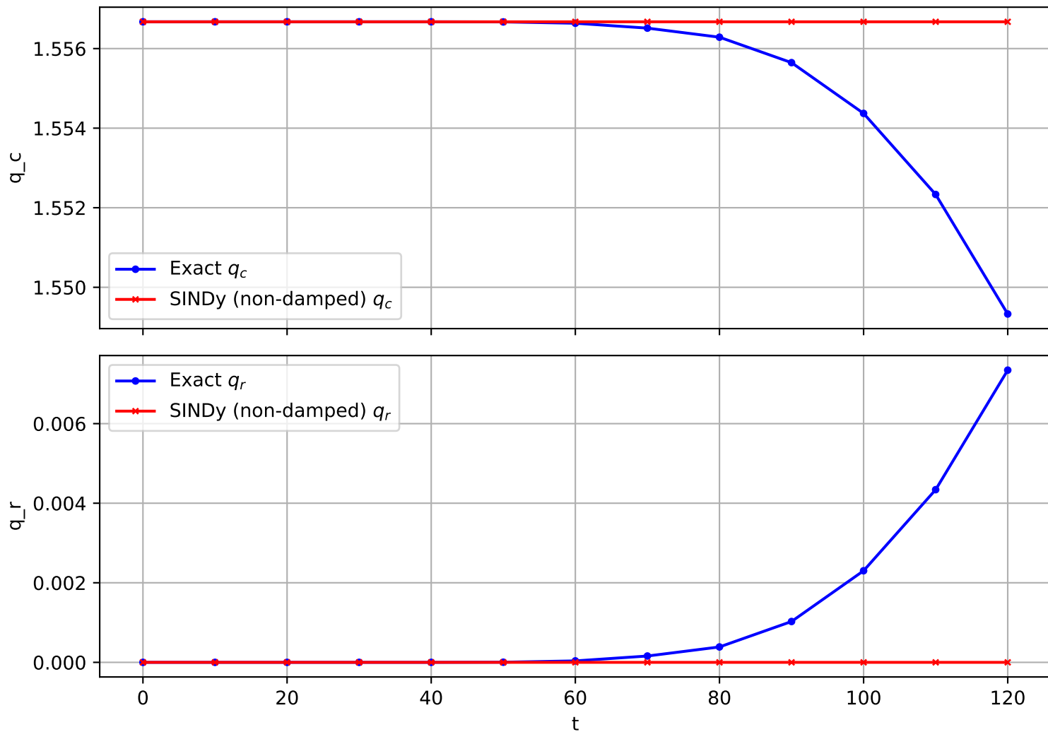
Trajectory 764 (non-damped)
