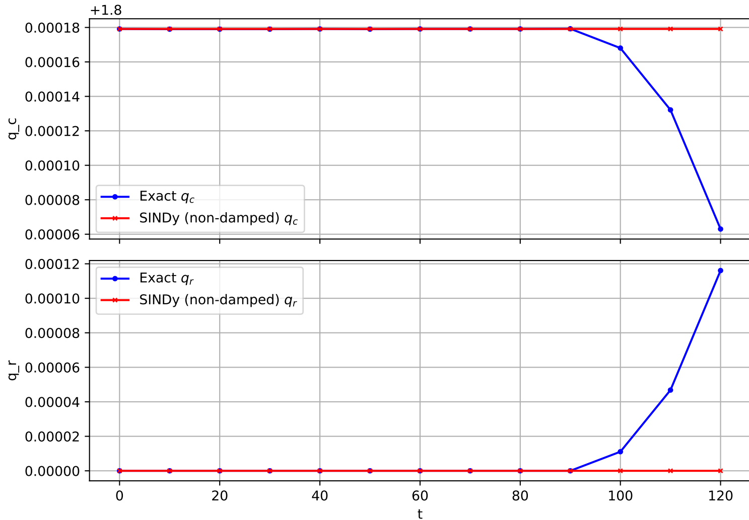
Trajectory 777 (non-damped)
