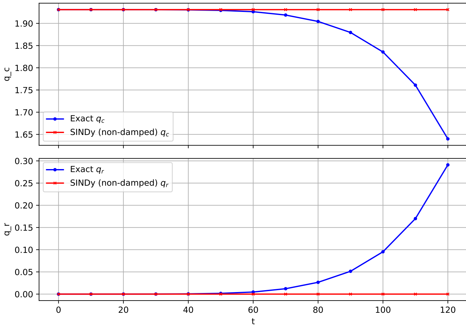
Trajectory 786 (non-damped)
