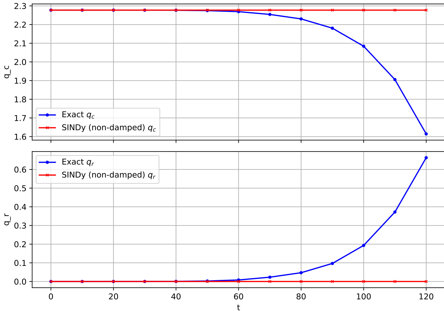
Trajectory 794 (non-damped)
