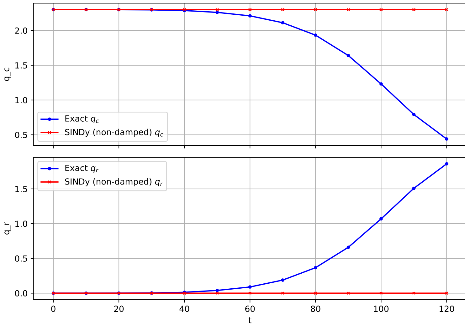
Trajectory 800 (non-damped)
