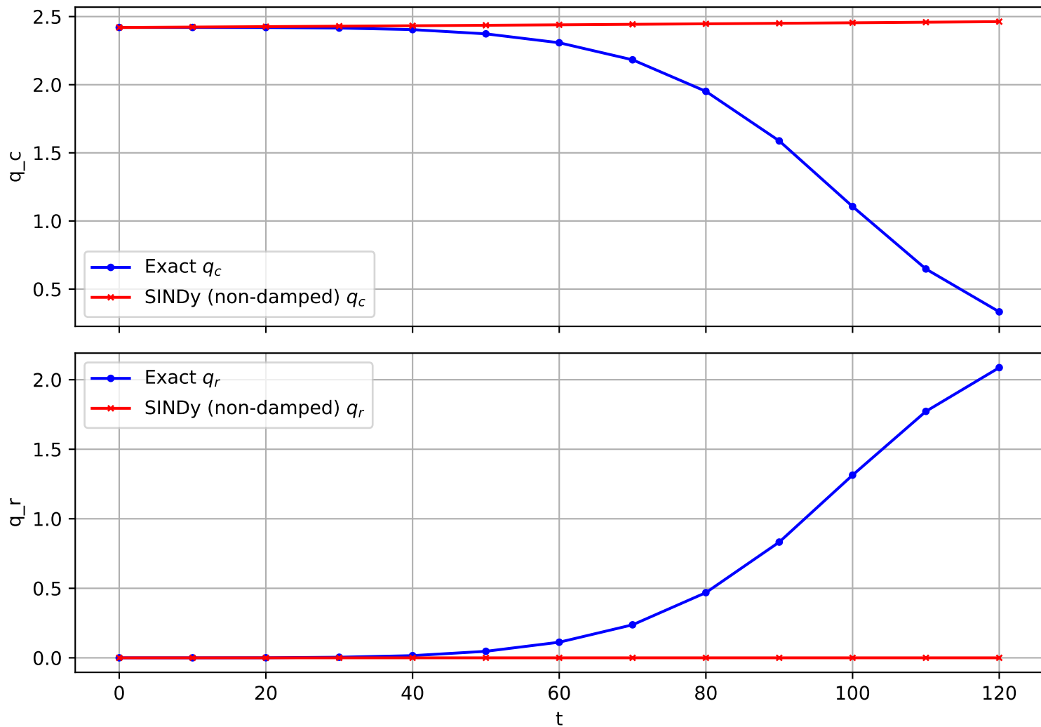
Trajectory 801 (non-damped)
