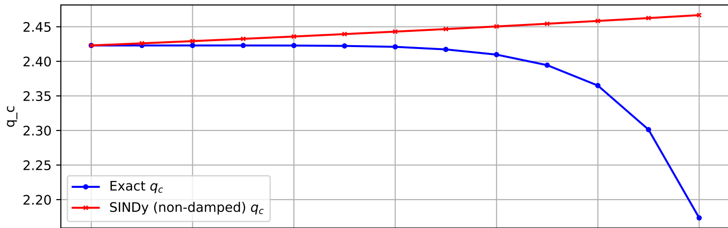
Trajectory 806 (non-damped)
