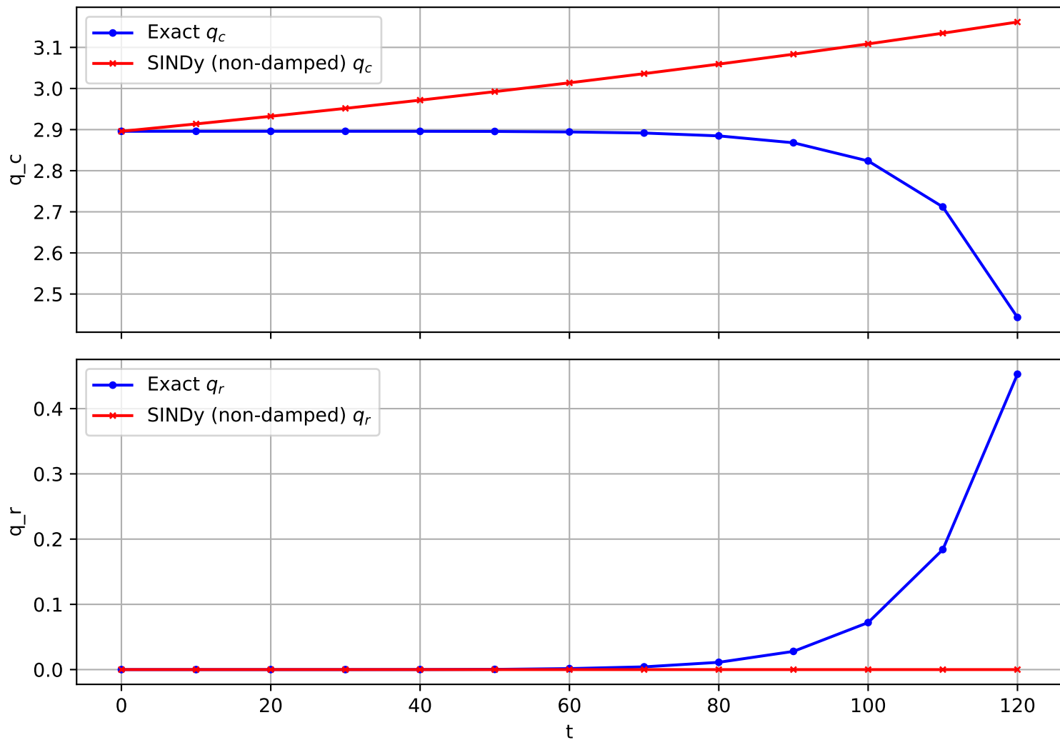
Trajectory 834 (non-damped)
