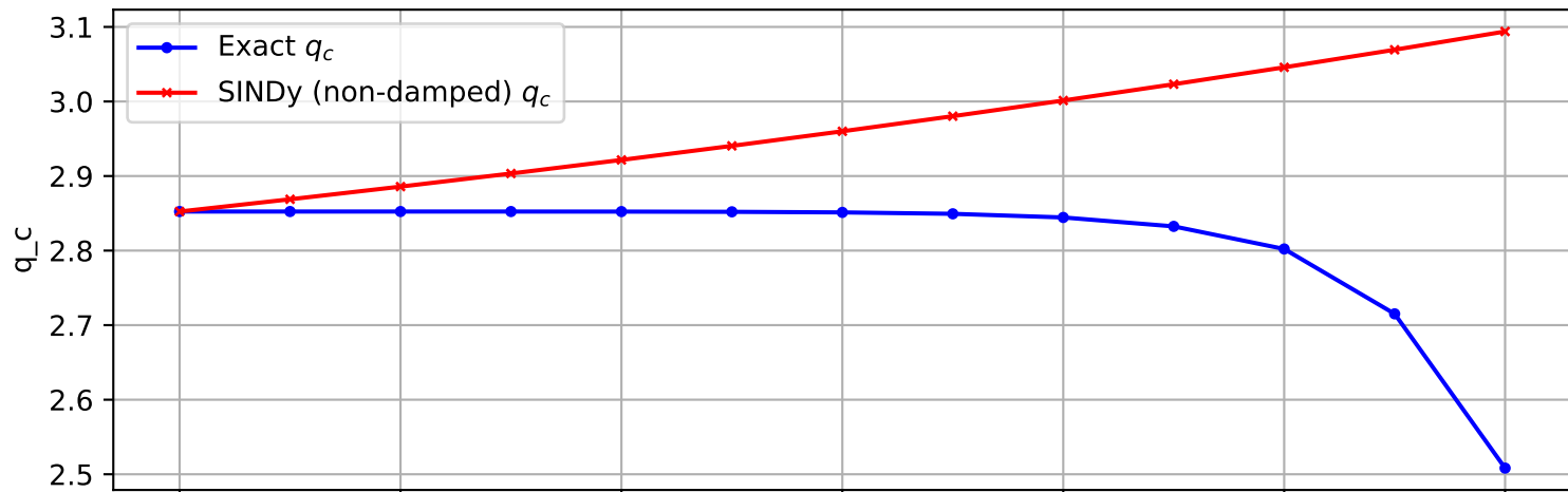
Trajectory 841 (non-damped)
