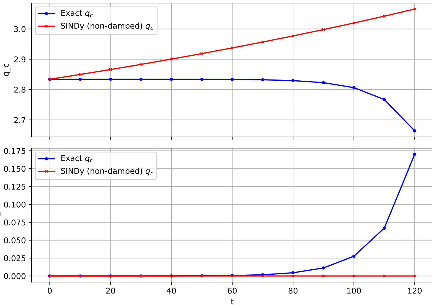
Trajectory 842 (non-damped)
