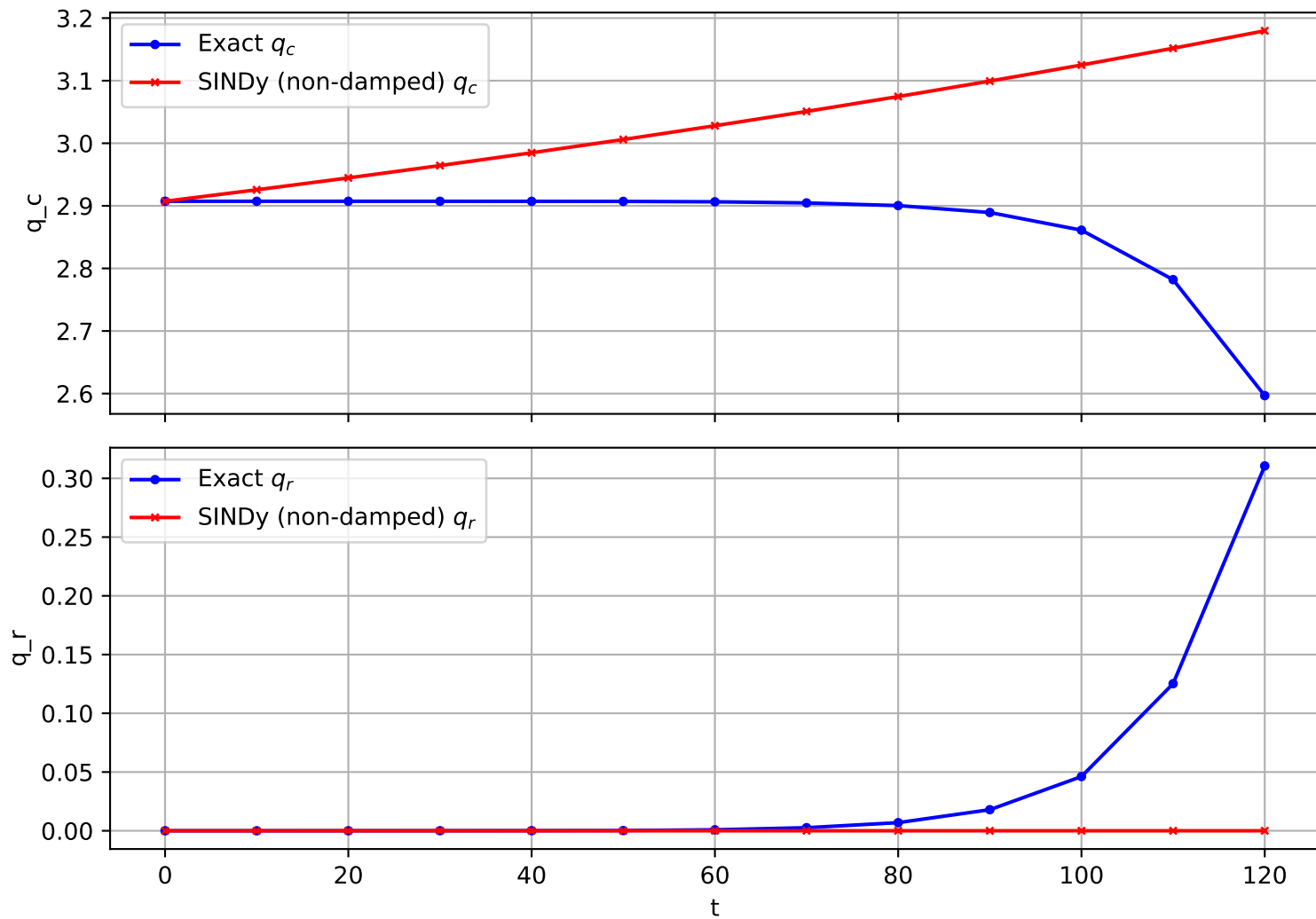
Trajectory 844 (non-damped)
