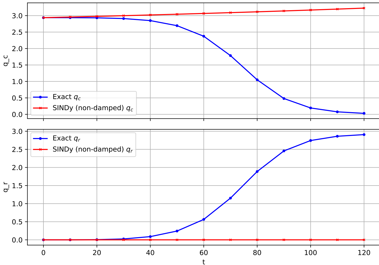
Trajectory 846 (non-damped)
