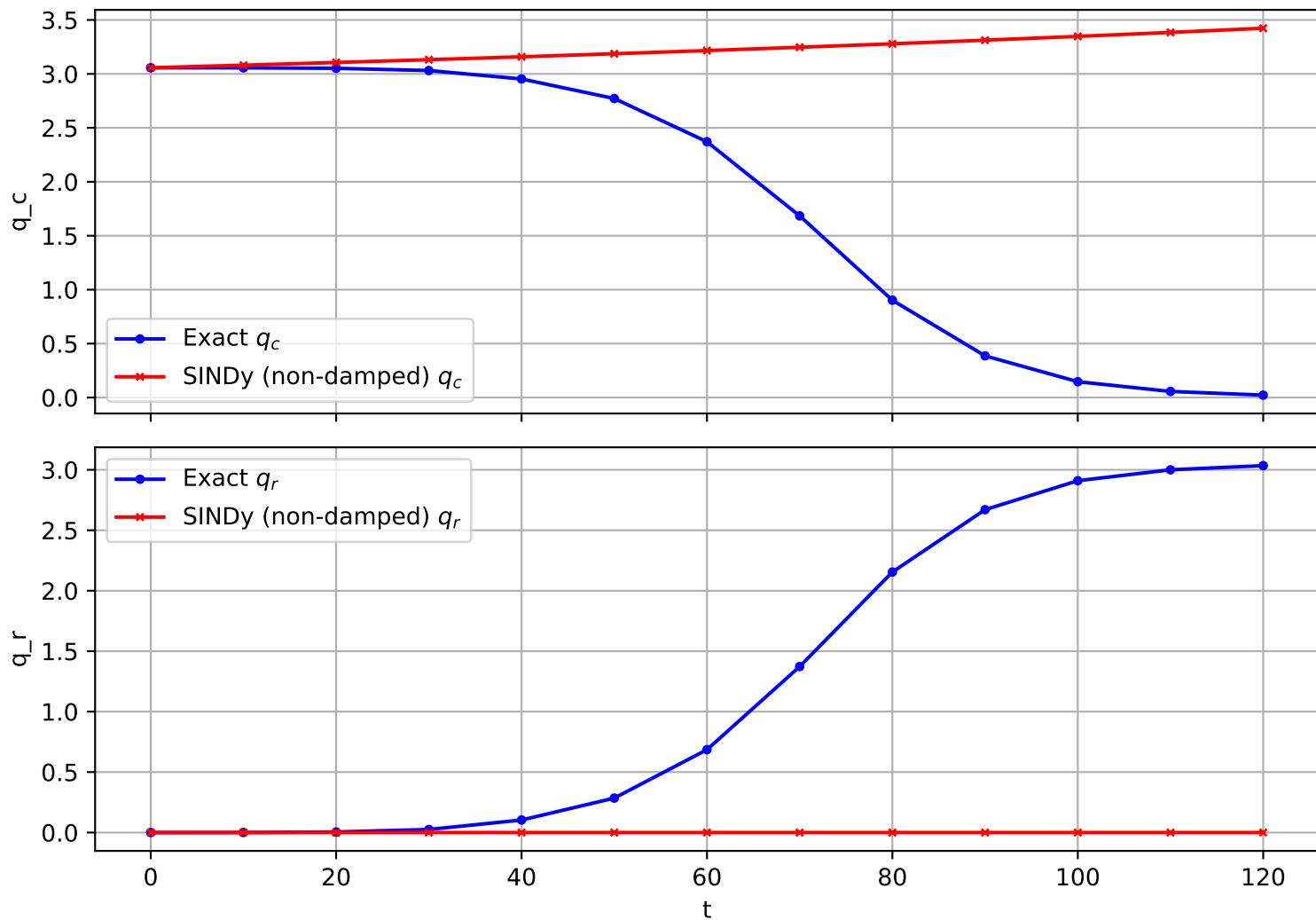
Trajectory 847 (non-damped)
