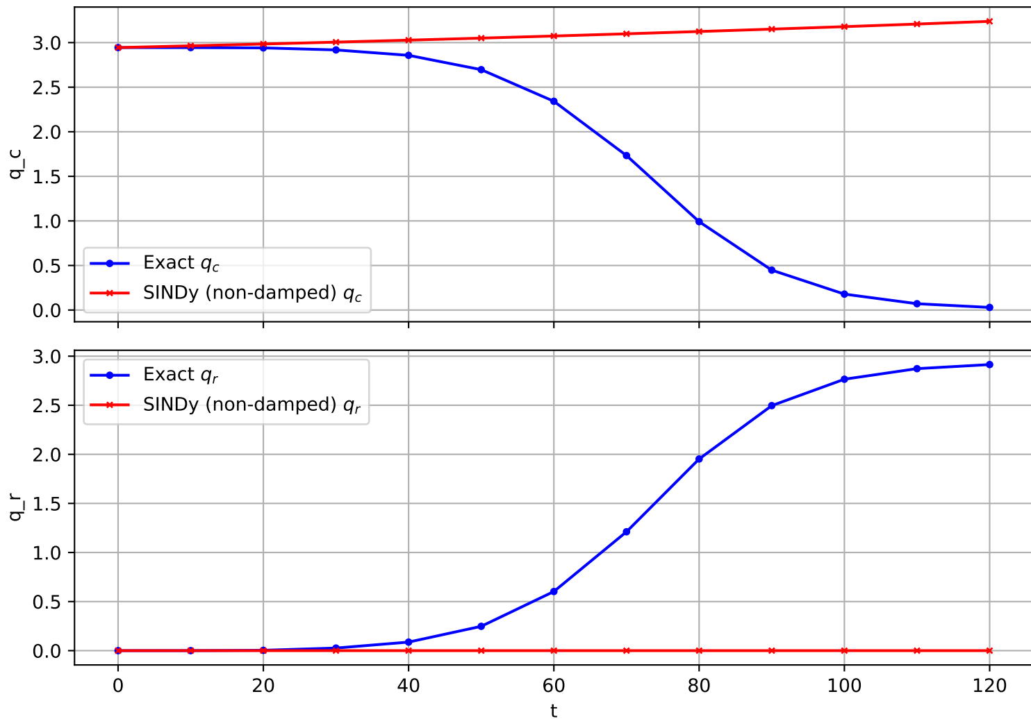
Trajectory 850 (non-damped)
