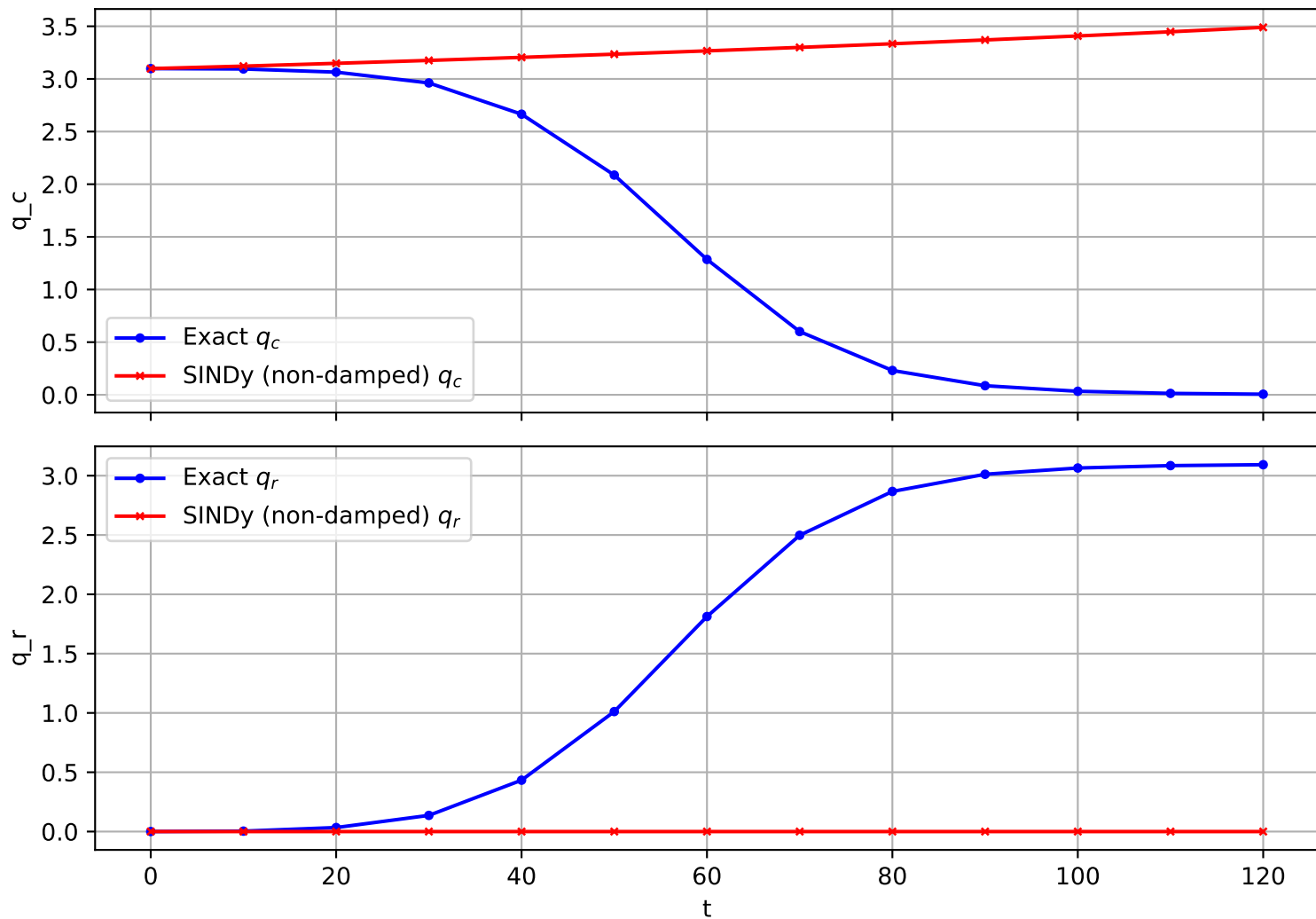
Trajectory 852 (non-damped)
