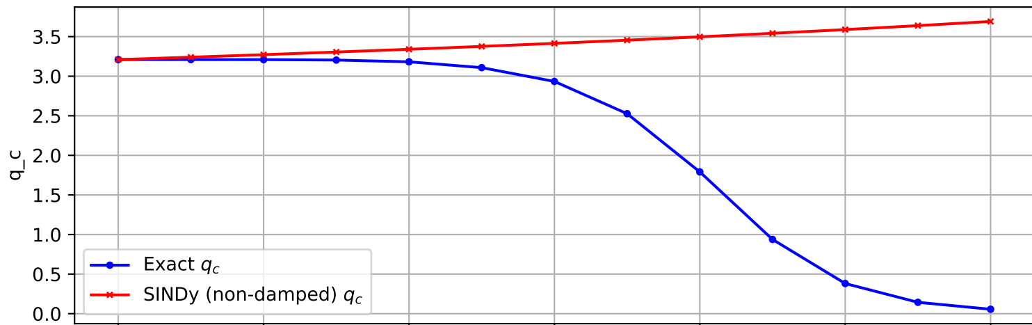
Trajectory 863 (non-damped)
