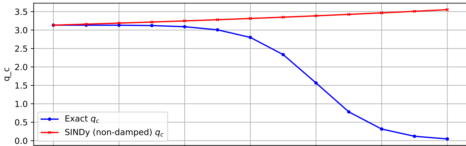
Trajectory 864 (non-damped)
