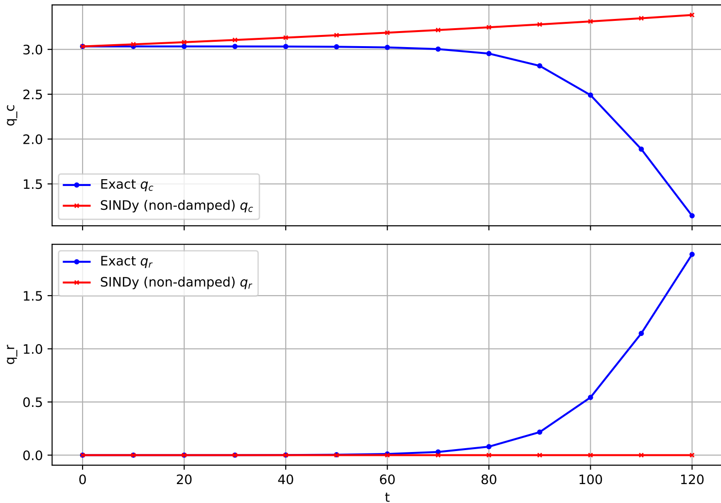
Trajectory 866 (non-damped)
