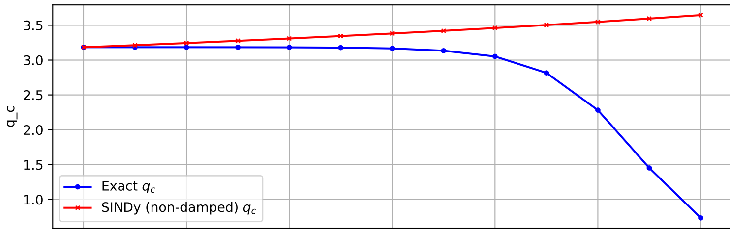
Trajectory 868 (non-damped)
