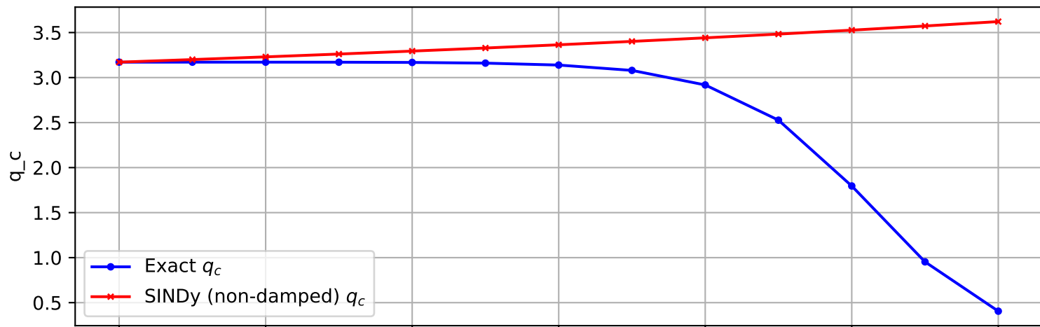
Trajectory 873 (non-damped)
