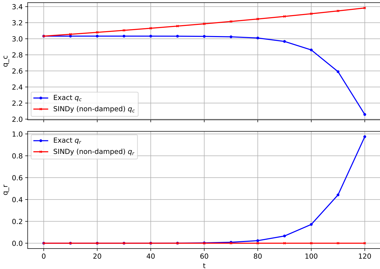
Trajectory 878 (non-damped)
