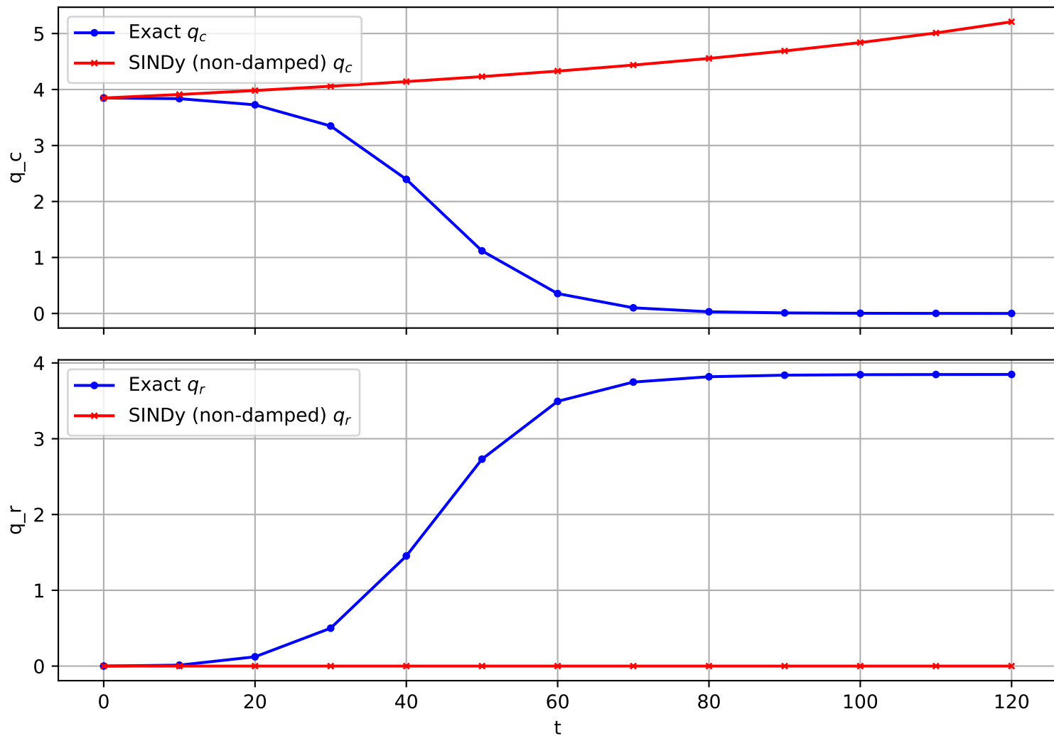
Trajectory 884 (non-damped)
