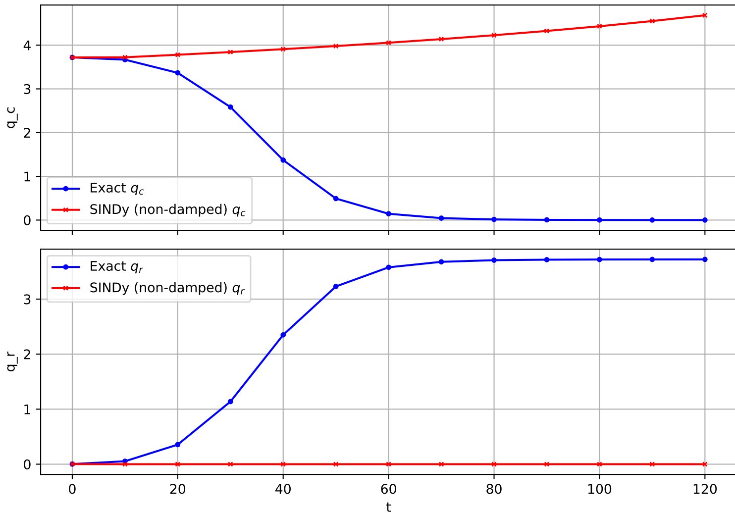
Trajectory 887 (non-damped)
