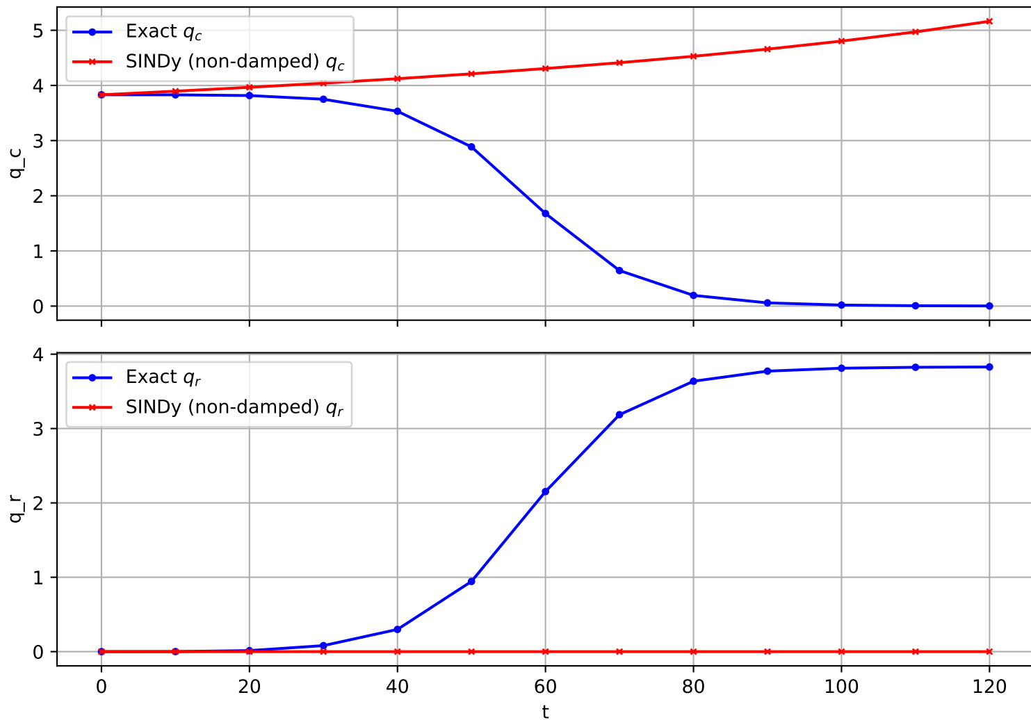
Trajectory 892 (non-damped)
