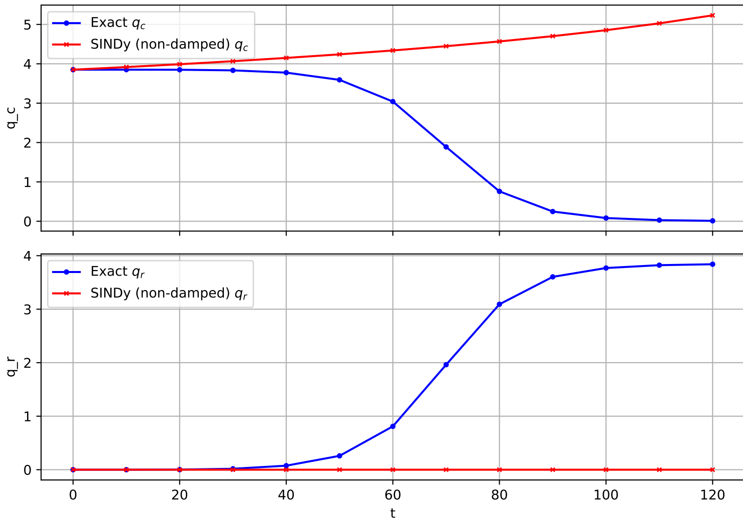
Trajectory 903 (non-damped)
