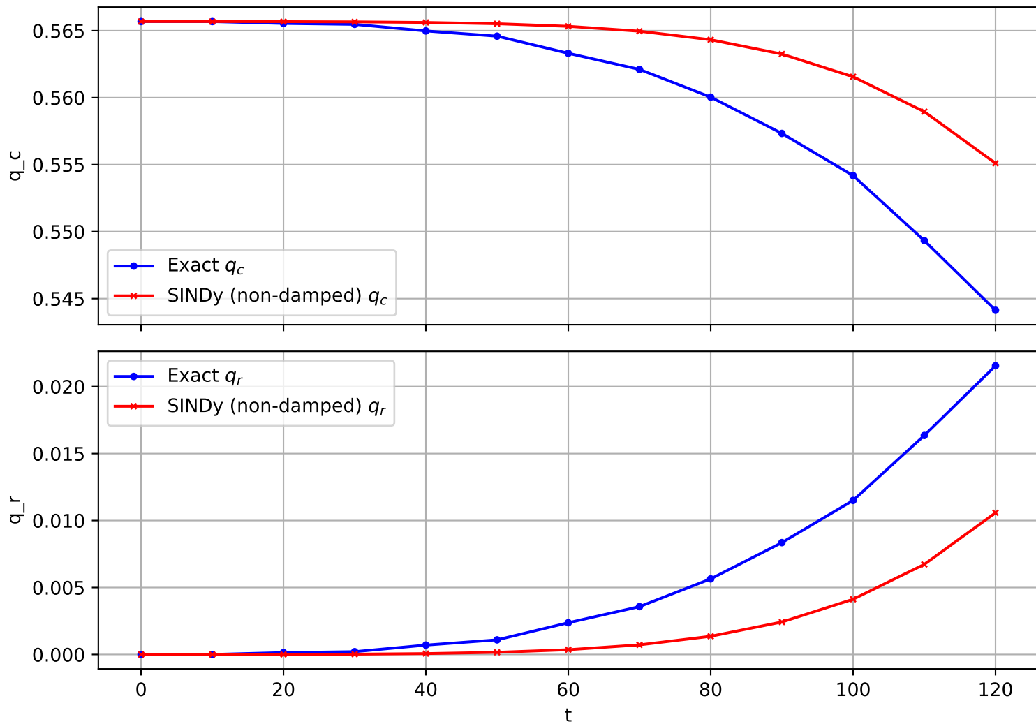
Trajectory 924 (non-damped)
