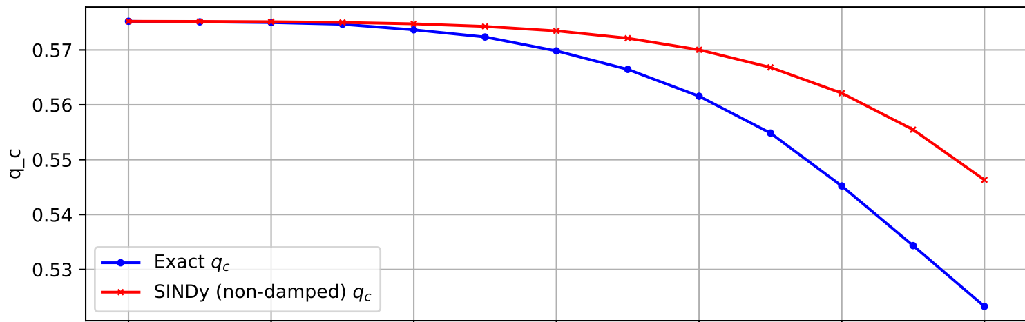
Trajectory 931 (non-damped)
