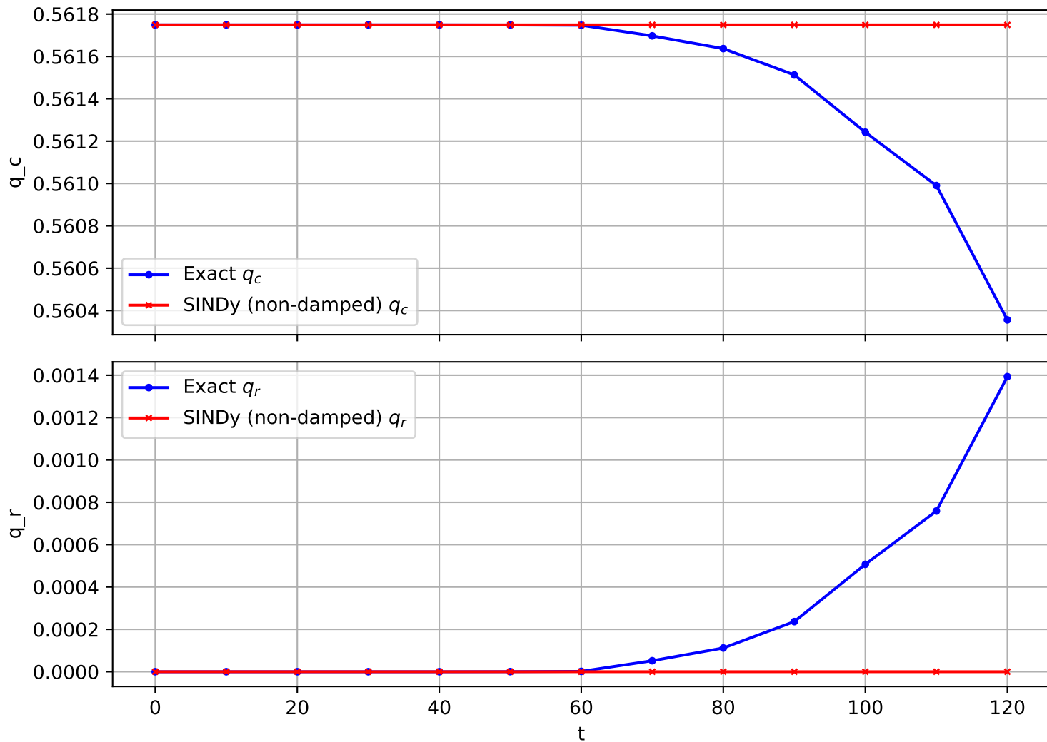
Trajectory 936 (non-damped)
