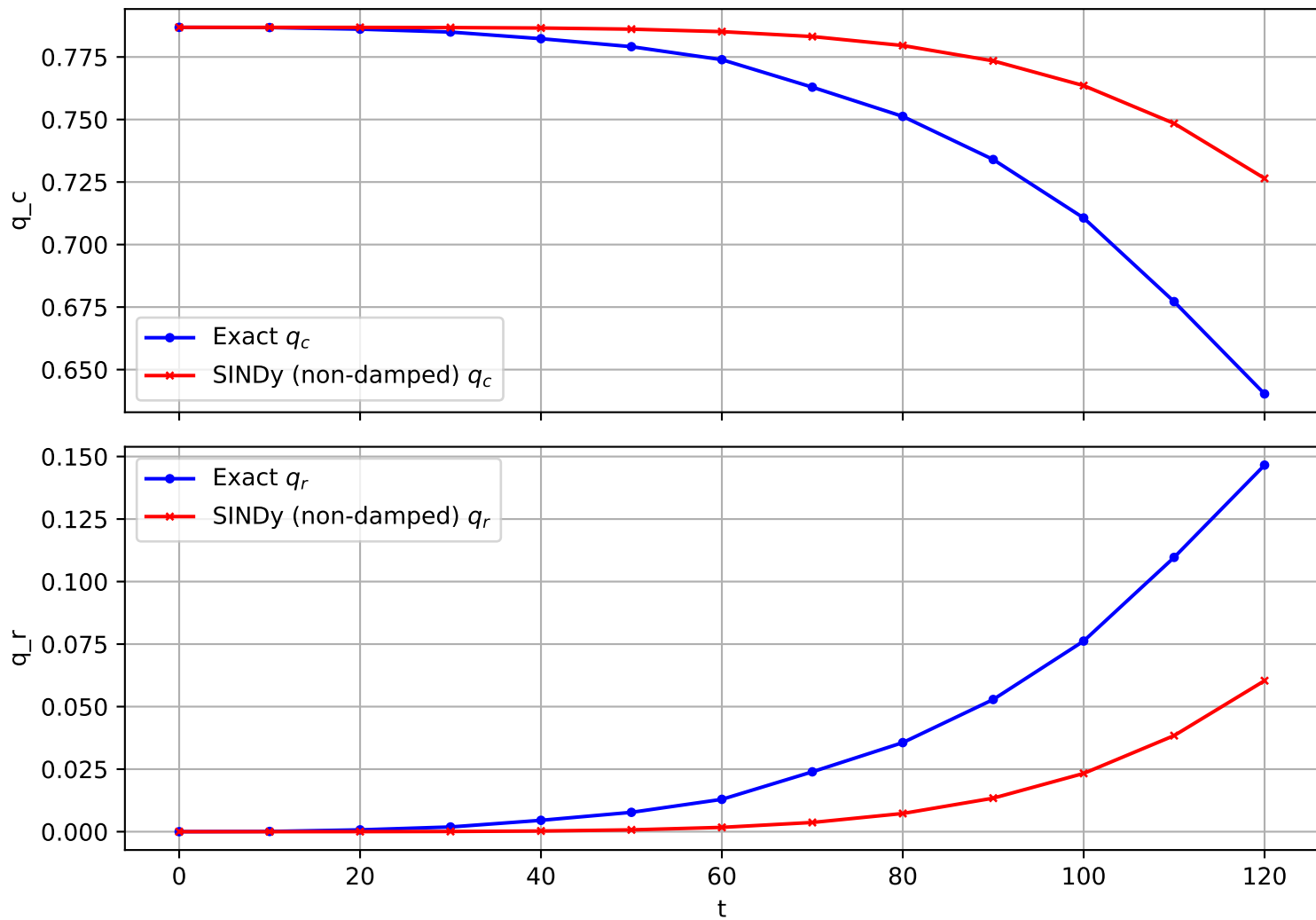
Trajectory 956 (non-damped)
