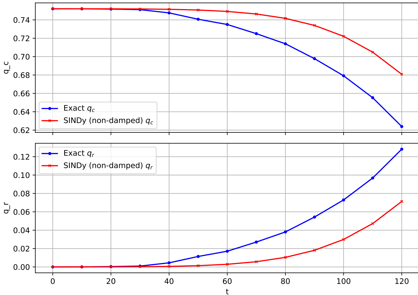
Trajectory 957 (non-damped)
